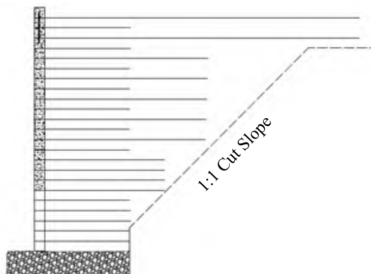
Section—Wing Wall
