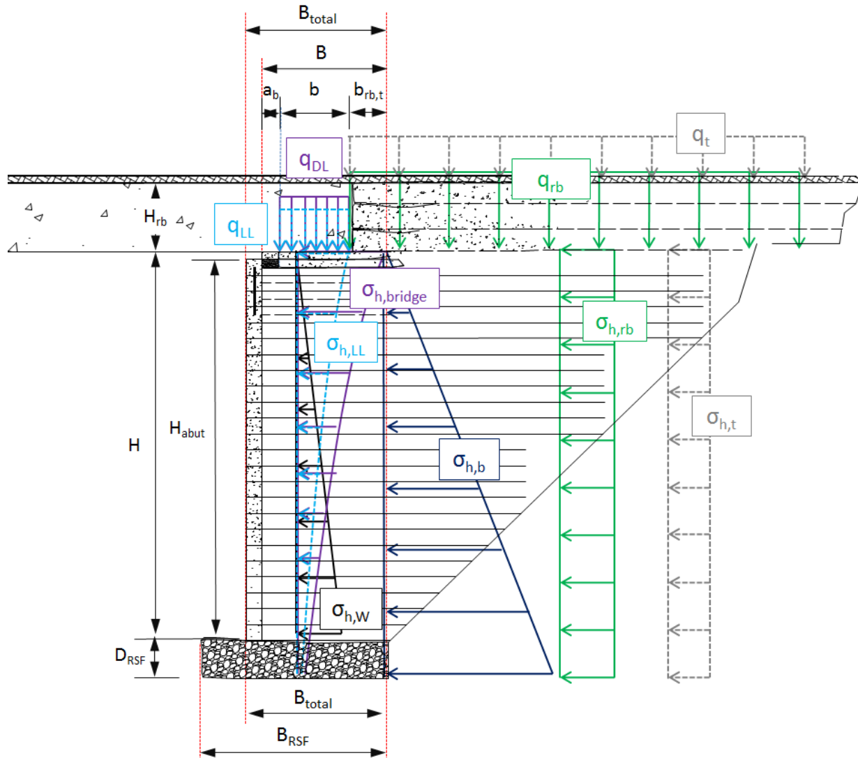
Figure 22. Illustration. Vertical and lateral pressures on a GRS abutment.
