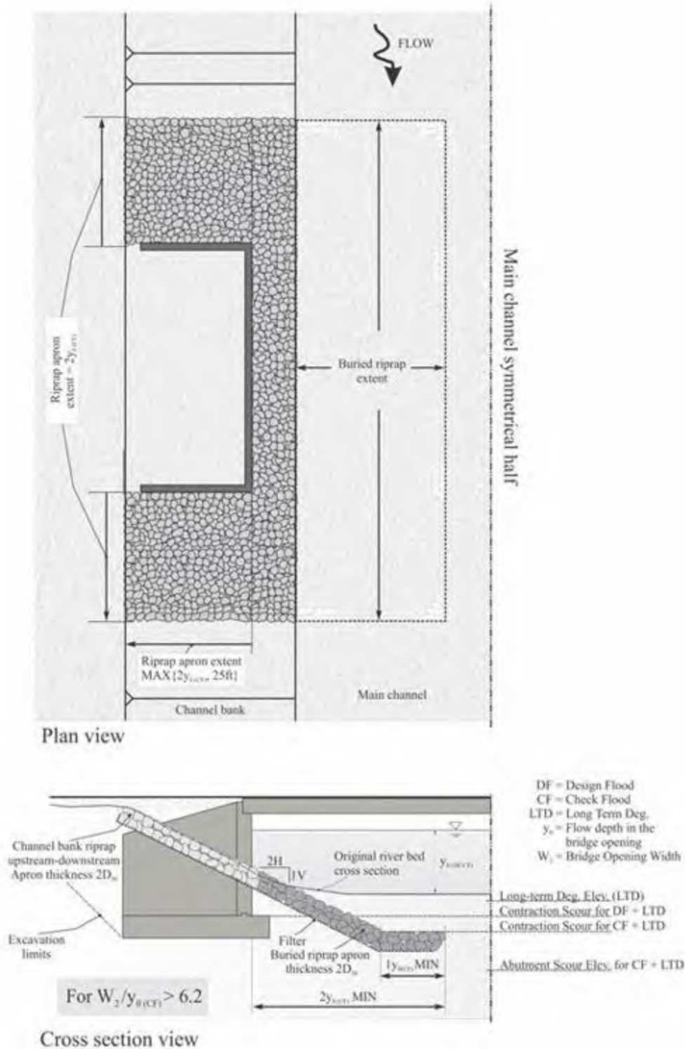
Figure 126. Illustration. Free-surface flow with wide-opening scour countermeasure (option 2).
